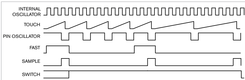
Figure 2 Representative waveforms that Figure 1 illustrates have a top-counter modulus of 3; a bottom-counter modulus of 12; and pin-oscillator periods of 3 and 6, respectively.
