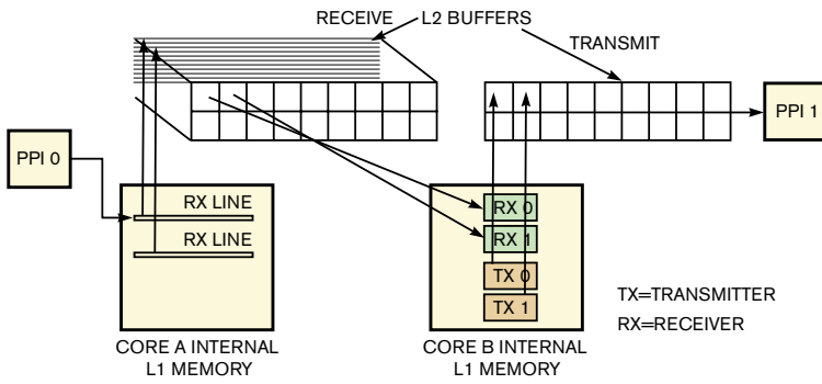
Figure 7 The data flow combines the line- and macroblock-processing frameworks.
