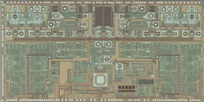
Figure 1 The Broadcom BCM2055 is a 4 \times 4 MIMO radio supporting the 802.11n draft specification. Note that both complexity and die area are not insignificant.
