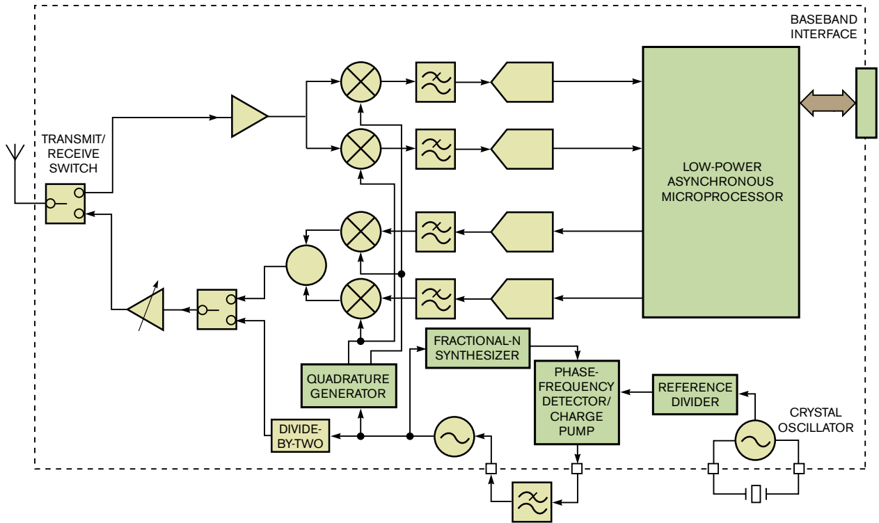
Figure 2 A typical two-way radio block shows the major functional subblocks (courtesy Berkeley Design Automation).
