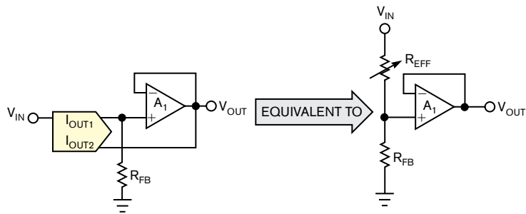
Figure 1 This simple circuit avoids a phase inversion and operates with a single supply. In this configuration, the DAC acts as a digitally programmable resistor.
