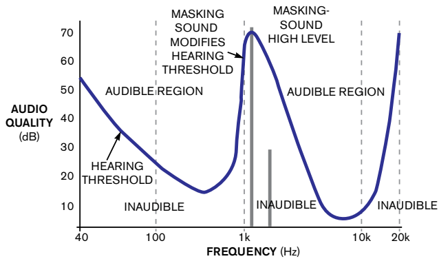
Figure 1 Psychoacoustic techniques enable discarding of substantial portions of the audio information without adversely affecting quality.
