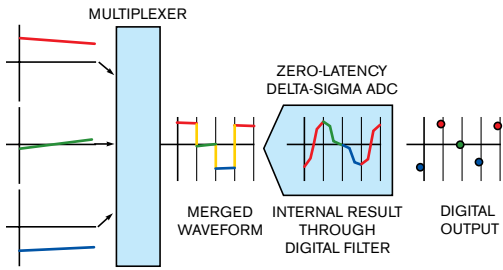
Figure 2 Switching dc signals into the ADC's input can contain high-frequency components.
