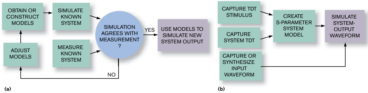
Figure 1 Measurement-based simulation requires acquiring or creating multiple models, such as transceivers, connectors, vias, and striplines. You must adjust the models to match the devices' behavior in a system and then combine them to simulate a new system (a). You can then combine captured or synthesized input waveforms with TDT measurements of the real system to simulate its behavior (b).
