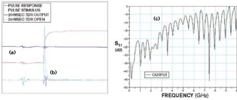
Figure 7 TDR yielded responses at an unpopulated board's output port and at the corresponding port of a populated board of the same design (a); derived impulse and impulse responses (b); and normalized S_{11} with the board effects removed (c).
