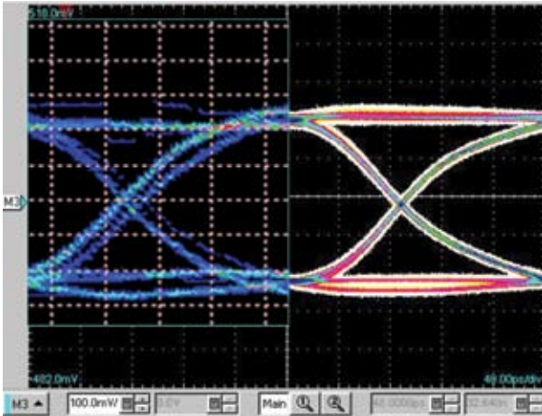
Figure 9 The output of a virtual transmission line (right) driven by a synthesized 4-Gbps PRBS waveform shows excellent agreement with a captured eye (left). These eye plots are for a 2^7-1 PRBS waveform with pre-emphasis from a Vitesse VSC3304HV crosspoint switch driving a 20-in. differential-transmission line.
