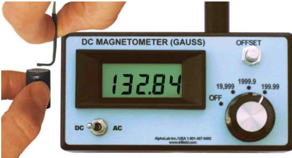
Figure 6 You can bend the sensor for this magnetometer into an L shape or keep it straight. It will withstand 1000 flexures (courtesy AlphaLab).
