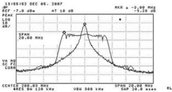
Figure 1 A Lexmark Profile of a modulated 66.666-MHz system clock (a) shows the relative EMI reduction for fundamental (b) and third-order harmonics (c).
