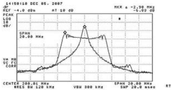
Figure 2 A triangular profile of a 66.666-MHz system clock (a) with a \pm 1.5\% center spread shows similar relative-EMI reductions for fundamental (b) and third-order (c) harmonics.
