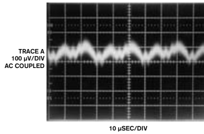
Figure 10 The controlled transition times dramatically lower noise to 150 \mu\text{V} p-p, a 20-fold improvement over that of Figure 7.
