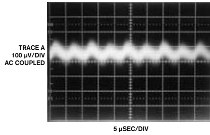
Figure 15 The output noise of the push-pull converter circuit in Figure 13 is barely discernible relative to the instrumentation's 100- \mu V noise floor. No wideband components appear in the 100-MHz measurement passband.
