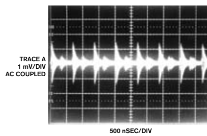
Figure 7 The switching-regulator harmonic in Figure 5 results in 3-mV-p-p output noise.
