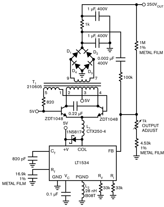
Figure 8 The LT1534 switching regulator features controlled transition times that minimize high-frequency harmonics and maintain low heat dissipation. The approach blends the benefits of switching- and linear-current-sink circuits.
