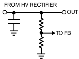
Figure A This collection of feedback network options begins with basic dc feedback.
