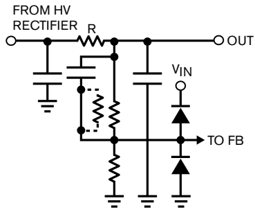
Figure D Enclosing resistor R in a dc loop lowers the output resistance. The feedback capacitor supplies a leading response.
