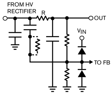
Figure E Moving the feedback capacitor to the filter further extends the leading response of Figure D's circuit.
