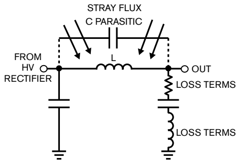
Figure F Replacing filter resistor R with an inductor lowers the output resistance but introduces a parasitic shunt capacitive path and is subject to stray-flux sensitivity.
