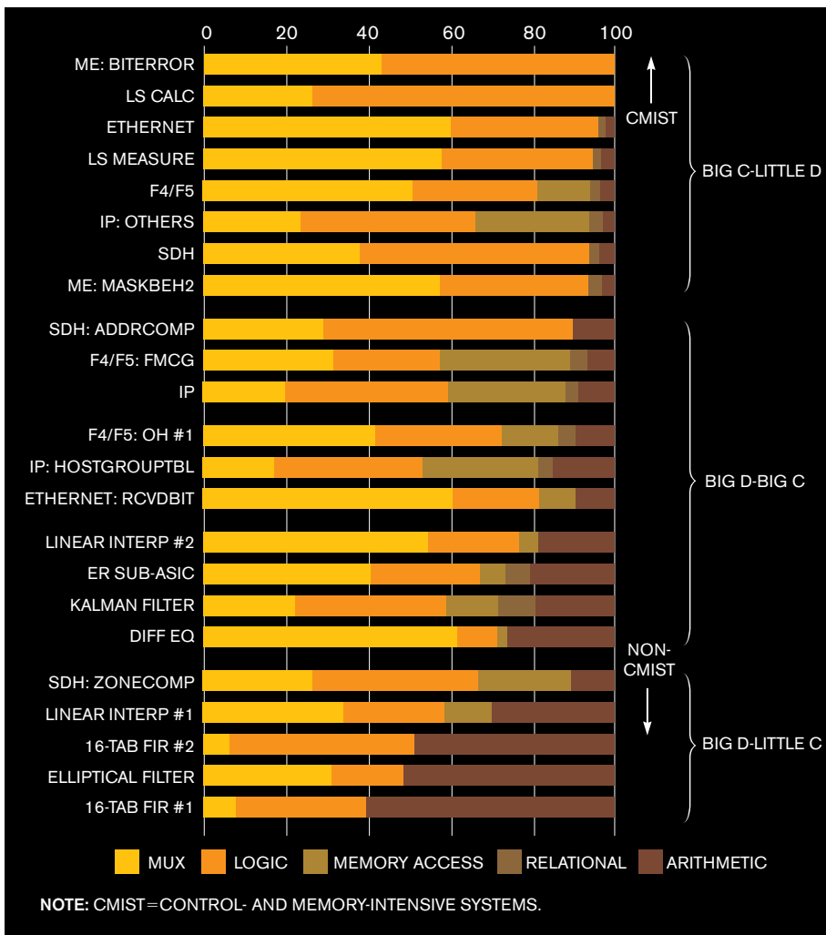
Figure A Tasks vary widely in their requirements for control, storage, and datapath functions. So, in some cases an ESL-synthesis tool's handling of control logic can be critically important, while in other cases it is not an issue at all.
