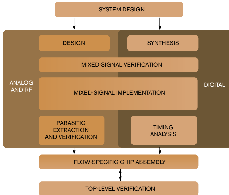
Figure 2 Breaking down the boundaries between analog and digital verification and implementation is the goal of Cadence's mixed-signal-design flow. The implementation stage, for instance, brings together Virtuoso and Encounter under OpenAccess, allowing each domain to understand the other without translation.
