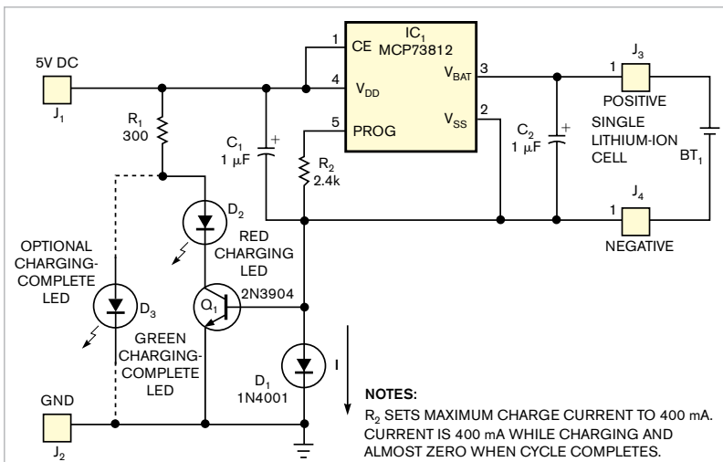
Figure 1 Adding a few components to a lithium-ion cell charger provides an indication of charging status.
