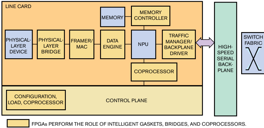
Figure 1 An FPGA can play a host of roles, but, in its most basic form, it is a programmable gasket or bridge between the framer and the NPU or between the NPU and the carrier-class-Ethernet switch.
