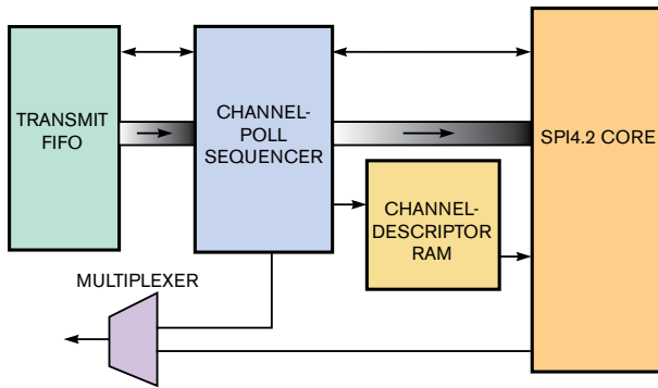
Figure 3 The scheduler could comprise a poll sequencer and a channel descriptor.
