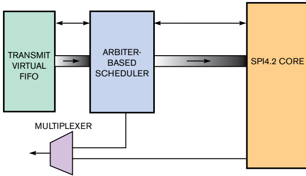
Figure 4 The objective of an arbiter-based architecture is to skip channels that have nothing to send and prioritize those channels that do.
