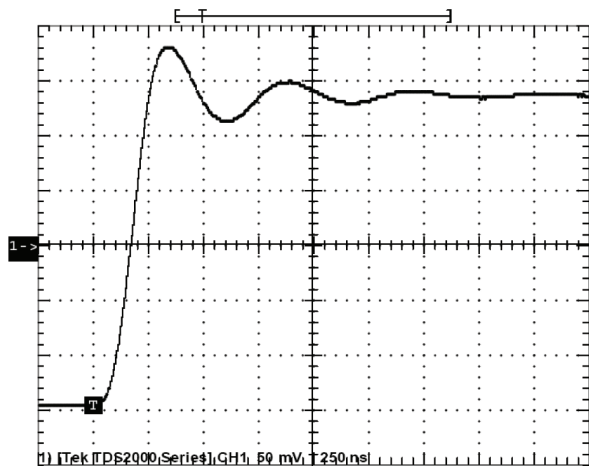
Figure 6 Measuring a 280-mV-p-p, small-signal step response (250-nsec/division, 50-mV/division scales) at V_{IN} with the OPA364 op amp yields an input resistance of 15\Omega and an input capacitance of 1500 pF.
