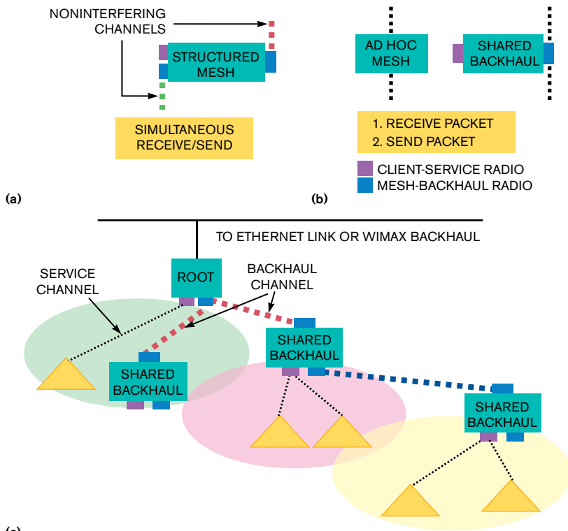
(c) Figure 3 You can build a separate radio structured mesh network with intelligent nodes and dynamic channel management (a) as an alternative to a radio mesh backhaul (b). The result is a network in which service and backhaul channels are both dynamically reallocated to minimize channel-interference effects. Locally changing the backhaul channels has no effect on the rest of the network (c) (courtesy Mesh Dynamics).
