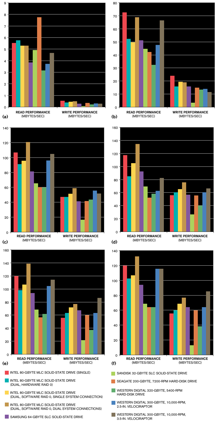
Figure 7 Sandra's Removable Storage test quantified drive performance as a function of file payload size: 512 bytes (a), 32 kbytes (b), 256 kbytes (c), 2 Mbytes (d), 64 Mbytes (e), and 256 Mbytes (f).
