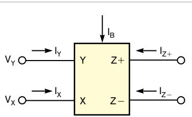
Figure 1 This dual-output current-controlled conveyor illustrates the quantities the equations use.
