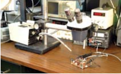
Figure D This Leica stereomicroscope was for sale at an electronics flea market for $200. The heavy base allows you to cantilever the microscope's head over your work area. A $100 dual-gooseneck illuminator from the same flea market sits on the base.
