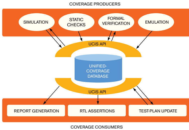
Figure A Coverage metrics come from many tools, and several kinds of clients consume them.
