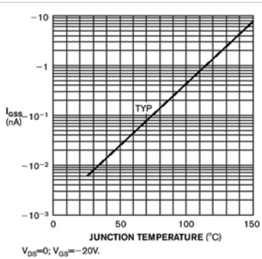
Figure 1 The reverse current of a PN-junction diode shows an exponential dependency over temperature; increasing the temperature by approximately 12K doubles the leakage.
