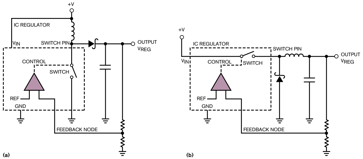
Figure 1 In both typical-voltage-step-up (a) and step-down converters (b), assume that the diode clamps the switch pin-voltage excursion to a safe limit.
