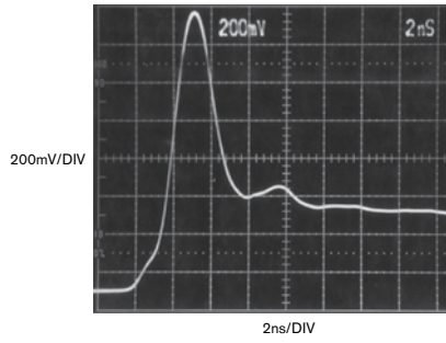
Figure 10 Diode 3 peaks at 1V above nominal 400-mV V_{FWD1} , a 2.5 \times error.
