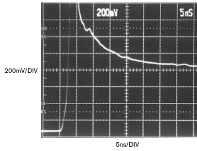
Figure 12 Diode 5 peaks offscale with extended tailing. Note the horizontal slower scale compared with figures 8 through 10.
