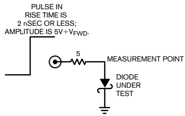
Figure 3 A conceptual method tests diode-turn-on time at 1A. The input step must have an exceptionally fast, high-fidelity transition.
