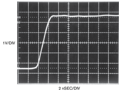
Figure 6 For a pulse-amplifier output into 5\Omega , the rise time is 2 nsec with minimal pulse-top aberrations.
