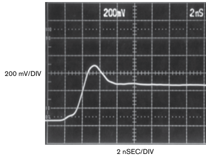
Figure 8 Diode 1 overshoots steady-state forward voltage for approximately 3.6 nsec, peaking at 200 mV.
