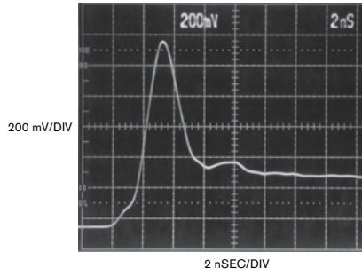
Figure 9 Diode 2 peaks at approximately 750 mV before settling in 6 nsec, more than twice the steady-state forward voltage.
