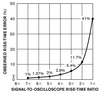
Figure A The measurement error rises rapidly as the signal-to-oscilloscope rise-time ratio approaches unity.
