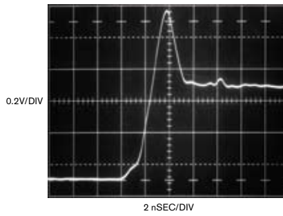
Figure B A typical diode turn-on viewed in a 2.5-GHz sampled bandpass displays 500-mV turn-on peak voltage.
