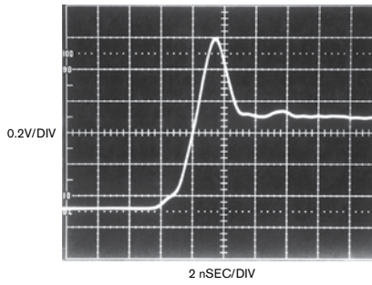
Figure C Figure B's diode turn-on observed in a 1-GHz real-time bandwidth has nearly identical characteristics, indicating adequate oscilloscope bandwidth.
