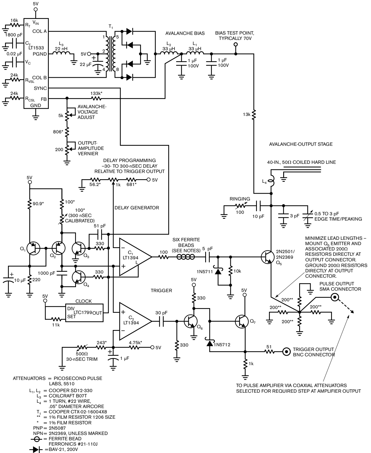
Figure A Variable delay triggers a less-than-1-nsec-rise-time pulse generator. The charge line at Q_5 's collector determines an approximately 10-nsec output width. The output-pulse occurrence is settable from before to after the trigger output.
