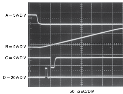
Figure C The pulse generator's waveforms are delay adjusted for the output pulse occurrence (Trace D) 25 nsec before the trigger output (Trace C). All other activity is identical to Figure B .
