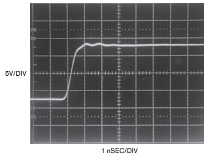
Figure D Excessive damping is characterized by front-corner rounding and minimal pulse-top aberrations. The trade-off is a relatively slow rise time.
