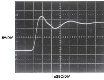
Figure E Minimal damping accentuates rise time, although pulse-top ringing is excessive.
