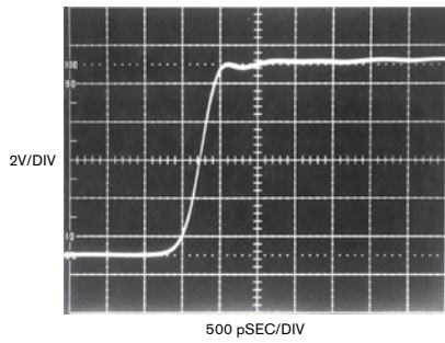
Figure F Optimal damping retards pulse-top ringing while preserving rise time.
