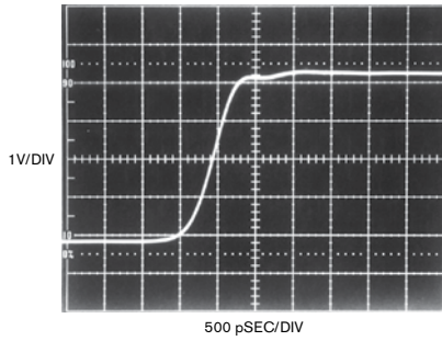
Figure B A 700-psec-rise-time pulse observed via a 50\Omega line and coaxial attenuator has good pulse-edge fidelity with controlled post-transition events.
